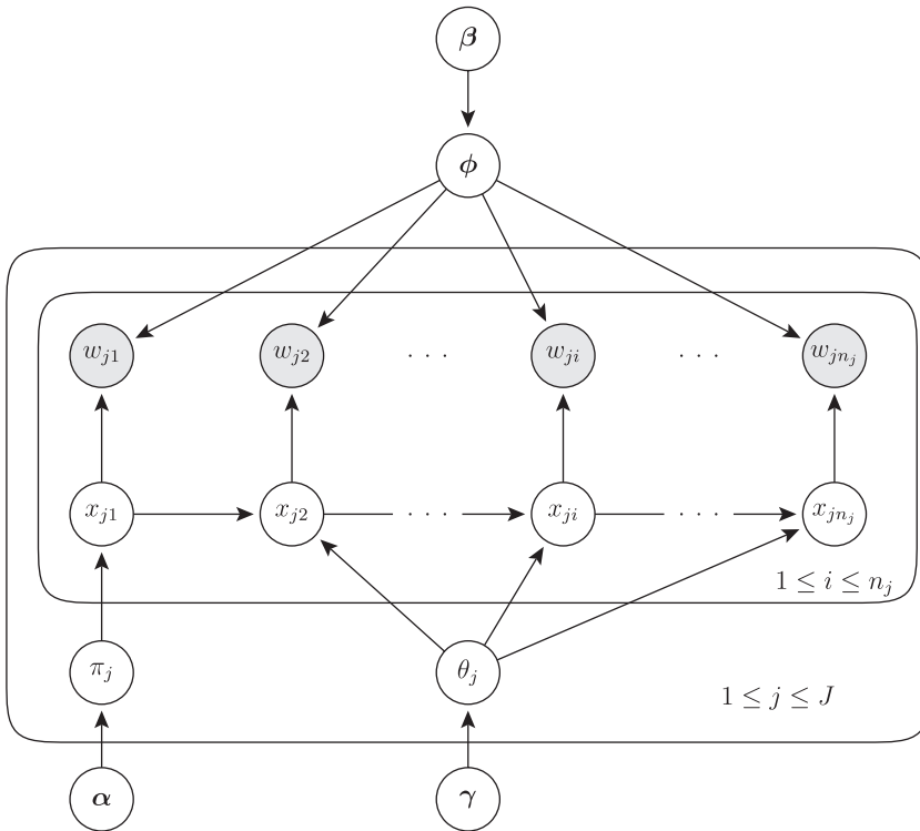
Fig. 2. A Bayesian network diagram for the Hidden Markov Topic model. As in the standard model, depicted in Fig. 1, each observed variable w_{ji} is assumed to be sampled from one of K topic distributions, collectively specified by \phi . Likewise, which one of these distributions is chosen is determined by the value of the unobserved variable x_{ji} . In the standard model, however, the latent variables x_{j1} \dots x_{jn_j} are drawn independently from a distribution \pi_j , which is specific to text j . In the HMTM by contrast, x_{j1} \dots x_{jn_j} are drawn from a Markov chain specific to the j th text. The parameters of this chain are \theta_j (i.e., the K \times K state-space mapping for chain j ) and \pi_j (i.e., the initial conditions for the j th chain). For all J texts, the parameters \theta_j and \pi_j are drawn from a common set of Dirichlet distributions. Each \theta_j is drawn from K -dimensional Dirichlet distributions, whose parameters are collectively specified by \gamma . Each \pi_j is drawn from a K -dimensional Dirichlet distribution \alpha . Also shown here is \beta , the parameters of a V -dimensional Dirichlet distribution from which the K topic distributions \phi are sampled.
