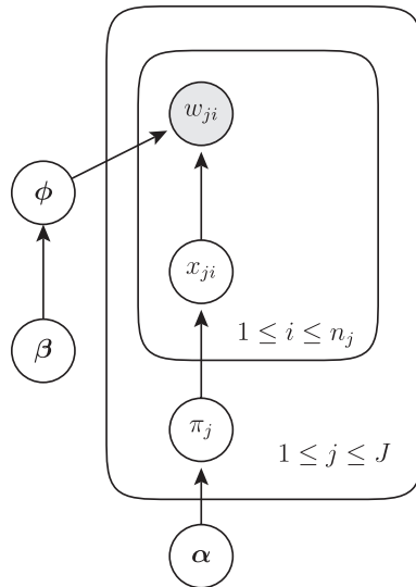
Fig. 1. A Bayesian network diagram of the standard Topics model described in Griffiths et al. (2007) and elsewhere. Details are provided in the main text. Note that \beta denotes the parameters of a V -dimensional Dirichlet distribution, from which each of K topic distributions is sampled.
