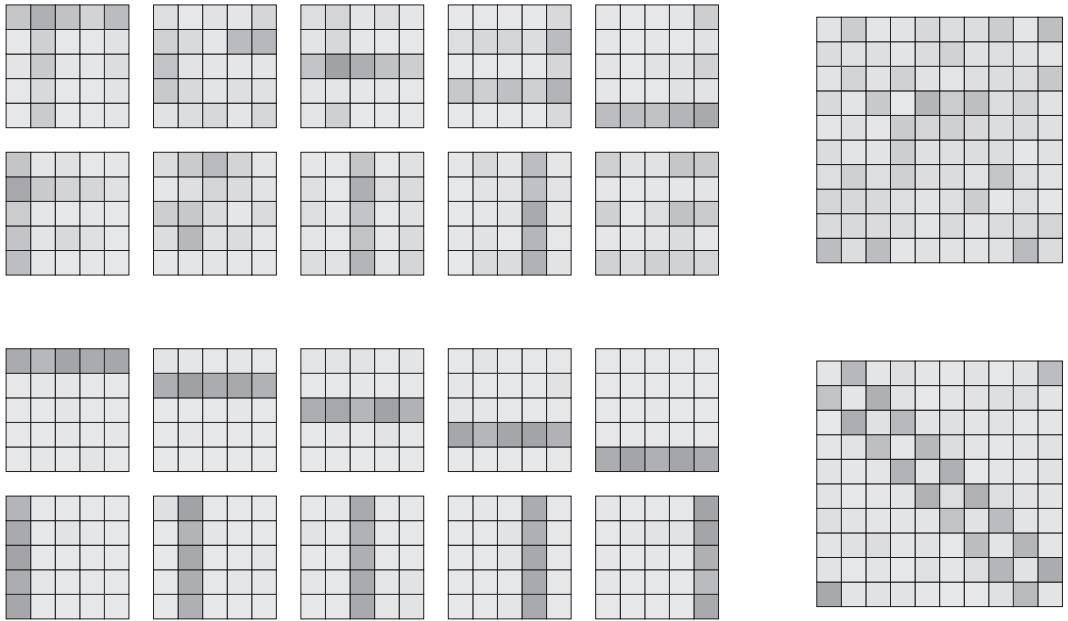
Fig. 3. Averages of samples from the posterior distribution over the topic distributions (left) and locations of the \gamma parameters (right). Shown on the top row are averages, over 10 draws, drawn after 20 iterations. Shown on the lower row are averages, again over 10 draws, taken after 100 iterations. Compare with the true parameters shown on the previous page.
